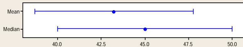
95% Confidence Intervals
